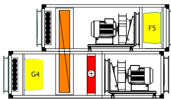
VEBAR CR...-P-KF4-KF5-NW-ER
